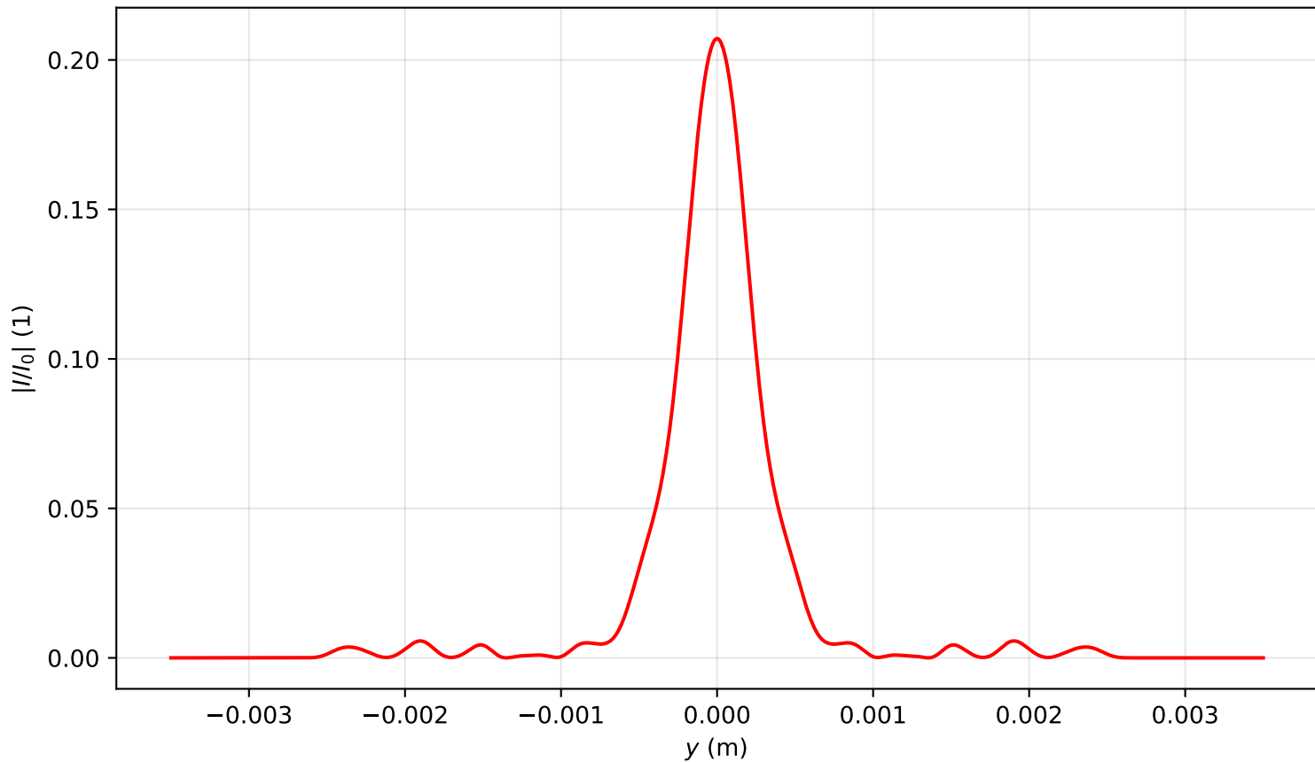
Intensity profile I(x=0, y, z=2.707)/I_0 , \text{Pin}=6.0\text{Pcr} , artificial time
